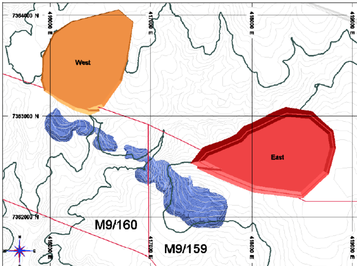
Figure 2: Yangibana Project – Yangibana North (M9/159) open pit and waste dump design.
